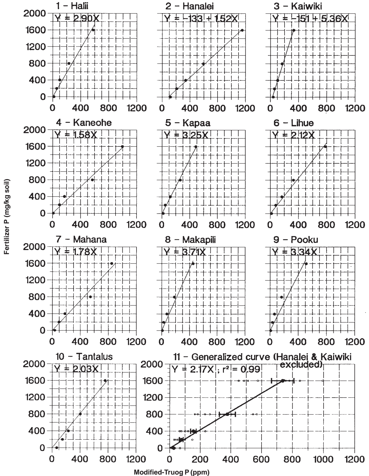
Figure 9-2. Relationship between fertilizer P applied and Modified-Truog P for some soils of Hawaii.
