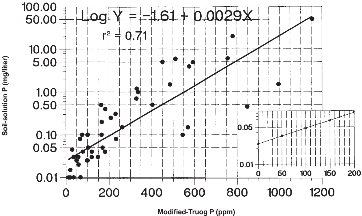
Figure 9-3. Relationship between soil-solution P and Modified-Truog P for soils of Hawaii.
