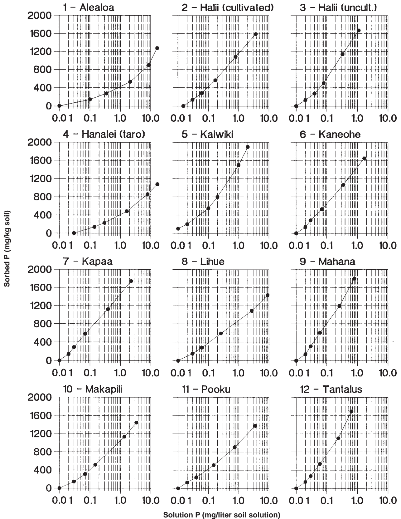
Figure 9-1. Relationship between sorbed P and soil-solution P in 12 soils of Hawaii.
