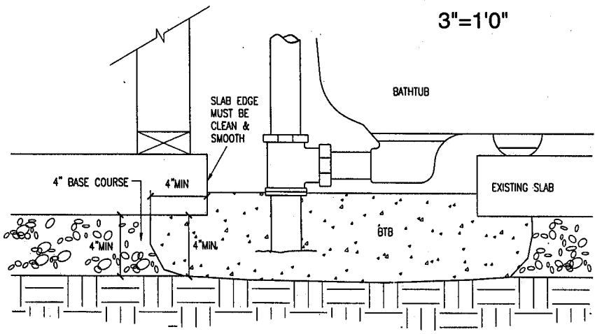
Fig. 9. Installation detail for BTB around the perimeter of an existing monolithic concrete slab.
