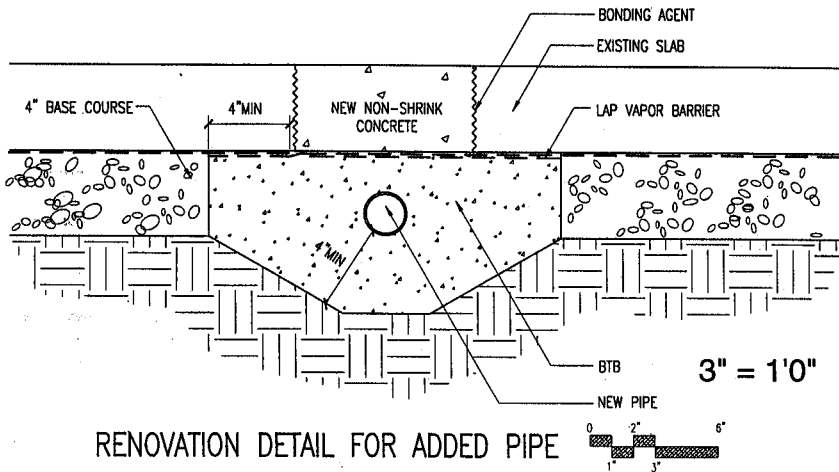
Fig. 11. Basaltic termite barrier detail for pipe renovations beneath concrete slabs.
