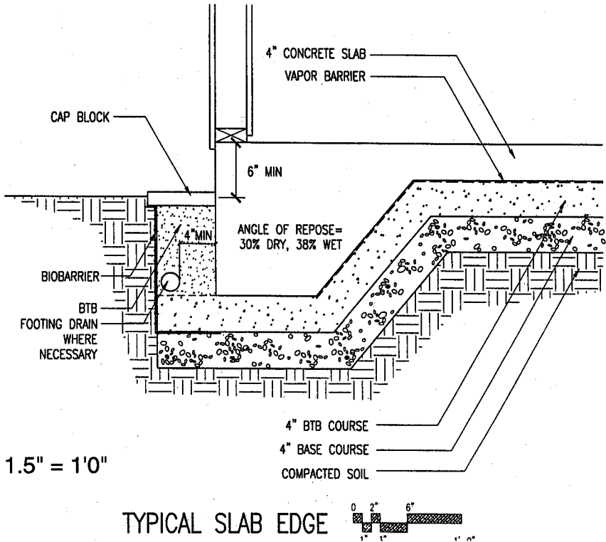
Fig. 1. Typical monolithic concrete slab edge showing the BTB detail, the termination point of the vapor barrier, and the use of BioBarrier.
