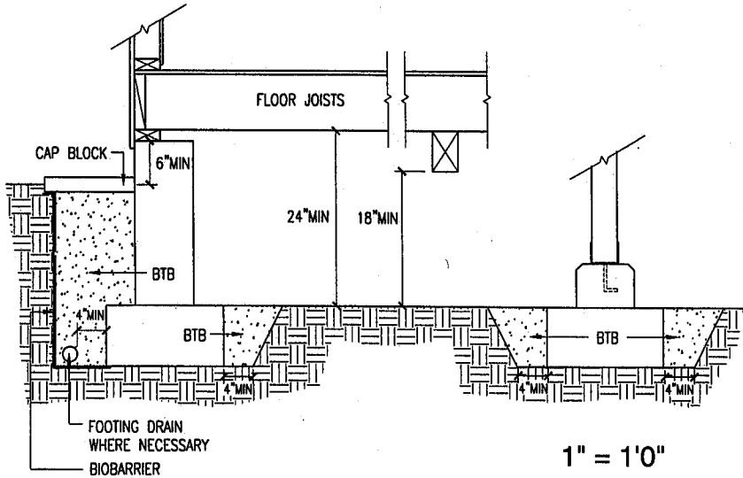
Fig. 7. Basaltic termite barrier installed as backfill for a stem foundation wall and around post-on-plier foundation blocks.
