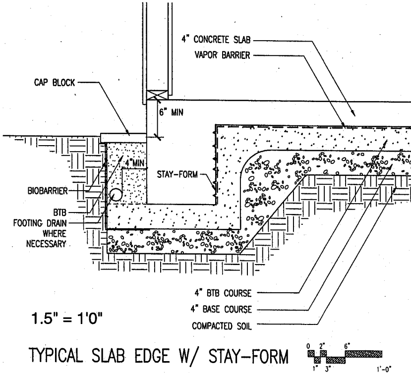
Fig. 5. Monolithic concrete slab edge with Stay-Form installed to increase the BTB angle of repose.
