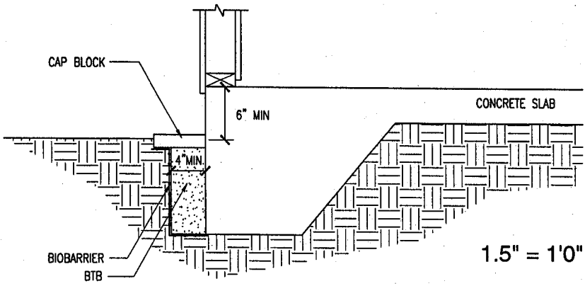
Fig. 9. Installation detail for BTB around the perimeter of an existing monolithic concrete slab.
