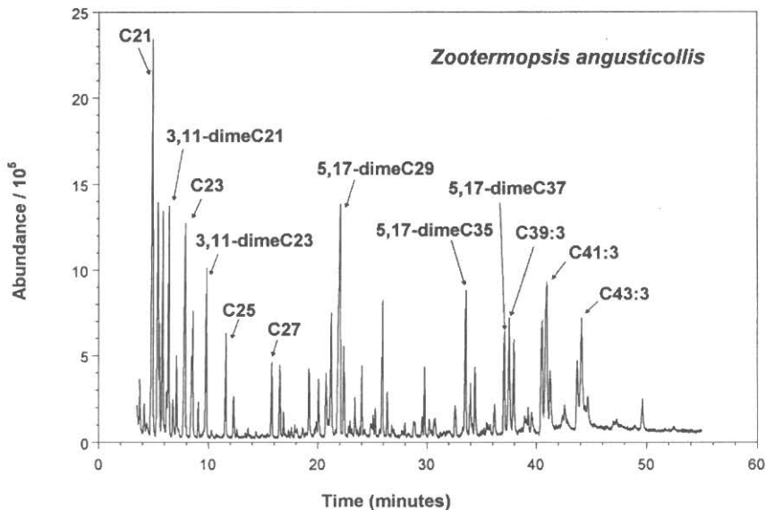
FIG. 6. Total ion chromatogram of the cuticular hydrocarbons from pseudergates of Zootermopsis angusticollis (Hagen) from Waiakoa Road, Kula, Maui, Hawaii.
