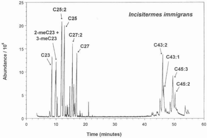
FIG. 2. Total ion chromatogram of cuticular hydrocarbons from pseudergates of Incisitermes immigrans Snyder from Coco Crater, Oahu, Hawaii.
