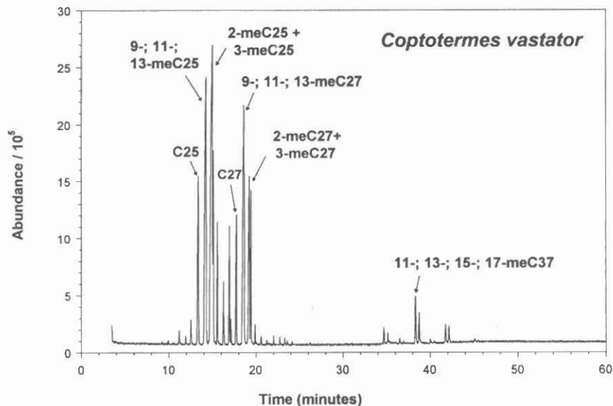
FIG. 8. Total ion chromatogram of cuticular hydrocarbons from workers of Coptotermes vastator Light from Guam.
