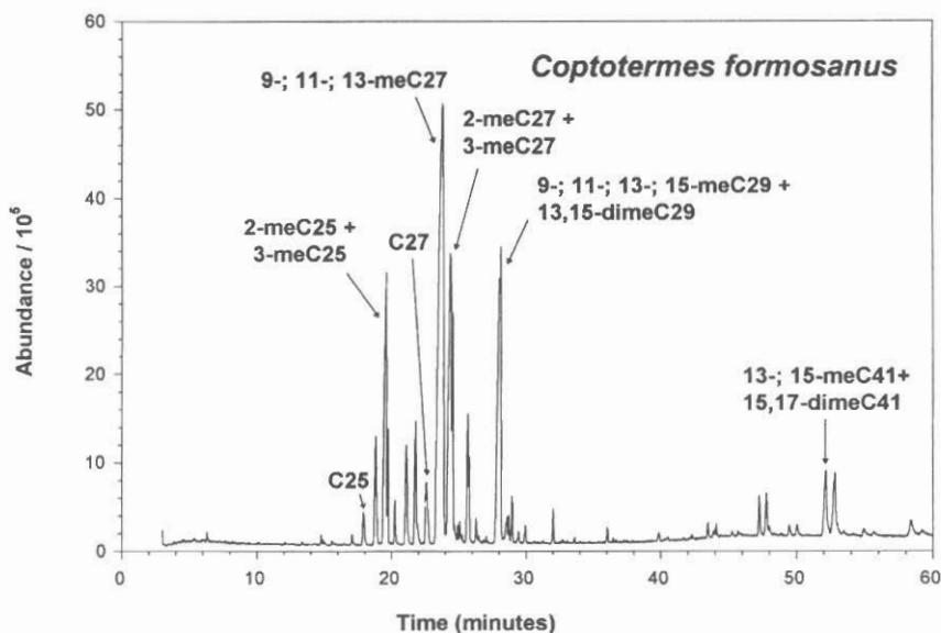
FIG. 4. Total ion chromatogram of cuticular hydrocarbons from workers of Coptotermes formosanus Shiraki from Honolulu, Oahu, Hawaii.
