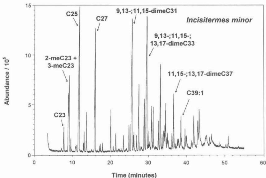
FIG. 7. Total ion chromatogram of cuticular hydrocarbons from pseudergates of Incisitermes minor (Hagen) from Waialua, Oahu, Hawaii.
