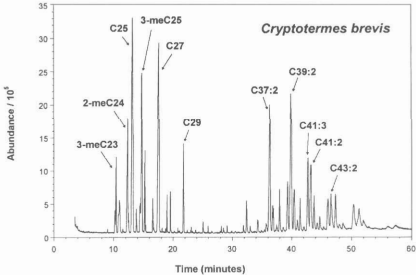
FIG. 3. Total ion chromatogram of the cuticular hydrocarbons from pseudergates of Cryptotermes brevis (Walker) from Honolulu, Oahu, Hawaii.
