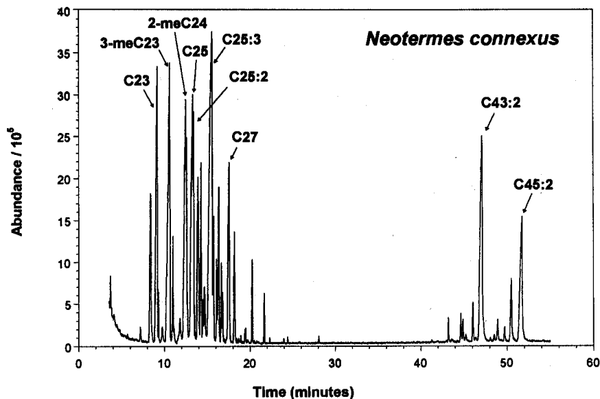
FIG. 1. Total ion chromatogram of the cuticular hydrocarbons from nymphs of Neotermes connexus Snyder from Iao Valley Lookout, Maui, Hawaii.
