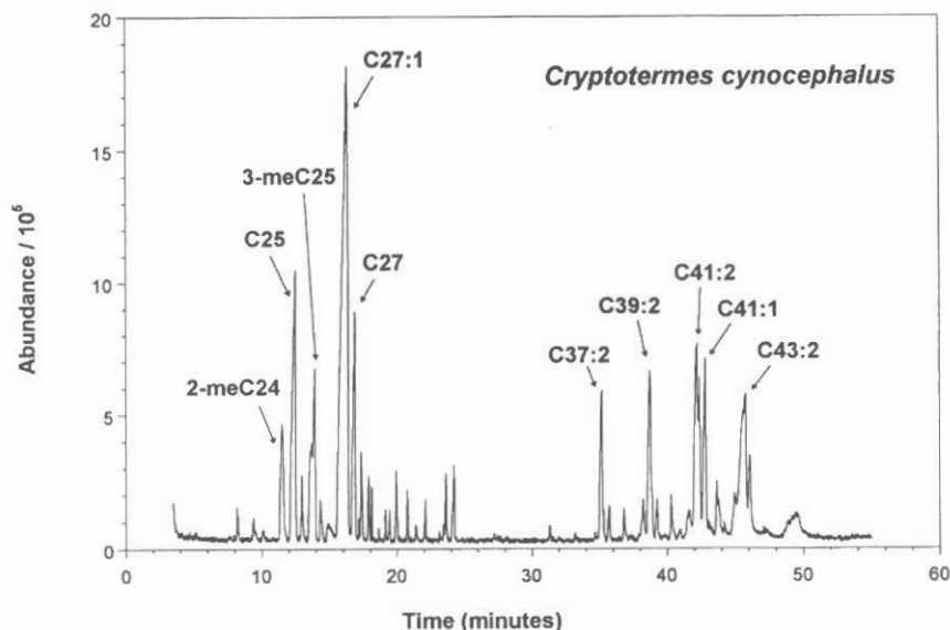
FIG. 5. Total ion chromatogram of the cuticular hydrocarbons from pseudergates of Cryptotermes cynocephalus Light from Waiahole Valley Road, Kamehameha Highway, Oahu, Hawaii.
