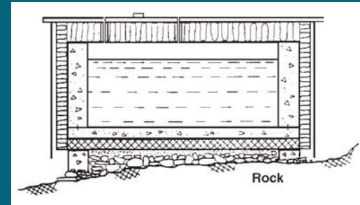
Frost protection of cistern on rock.
