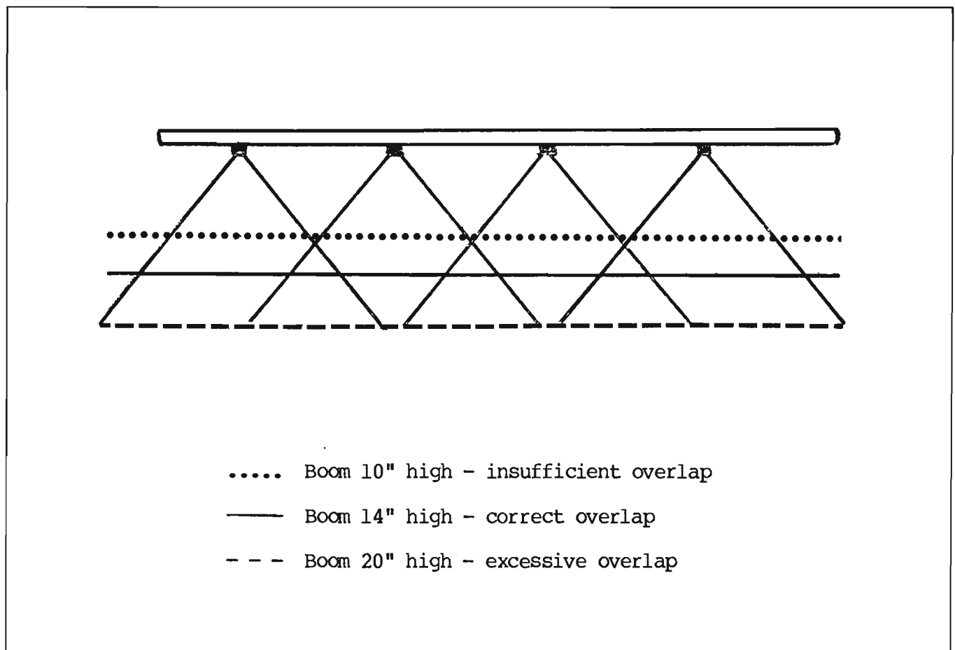
Figure 2. Effect of boom height on spray pattern. Nozzles are 80° angle flat-fan type spaced 18 inches apart on the boom.
